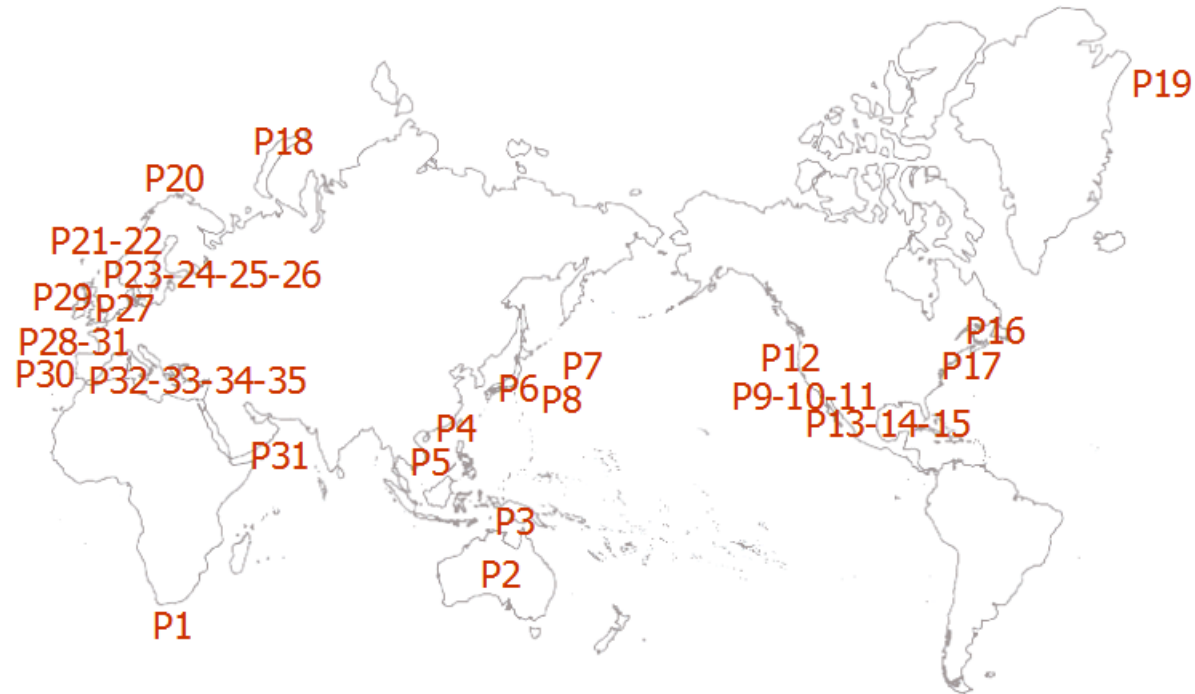
Figure 1: Coastal & Shelf Seas downscaling projects linked to GODAE
